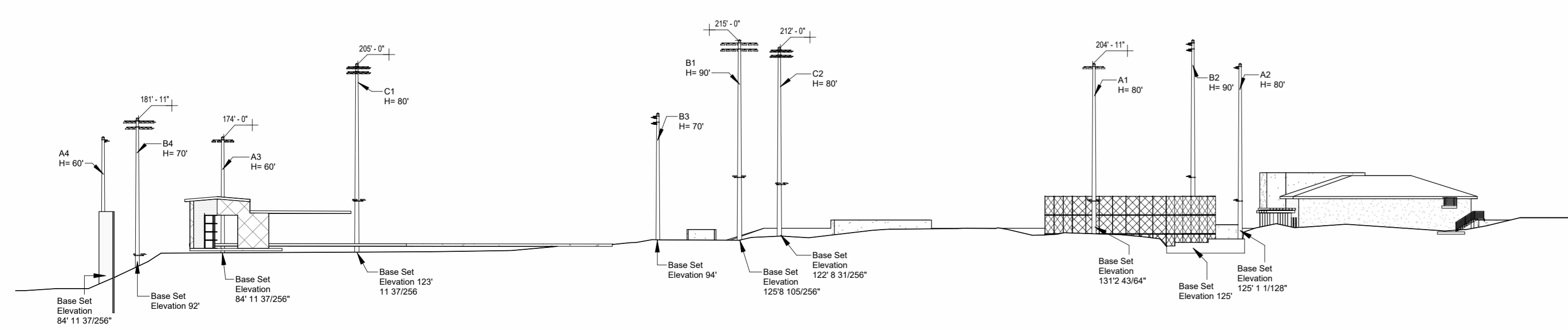
2 Section 16 Pole Height 1" = 40'-0"
